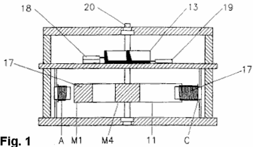
Fig.1 shows a cross-sectional front view of a rotary device as a control therefore in accordance with a first embodiment of the invention;
